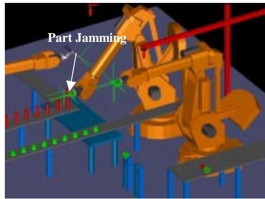
Figure 2: Part jamming at the 1 st station
